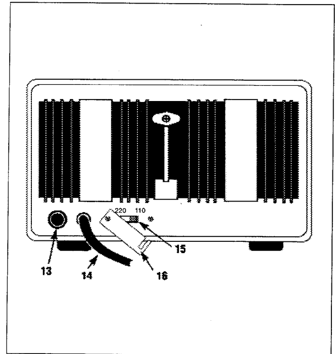
Figure 2. Rear Panel
