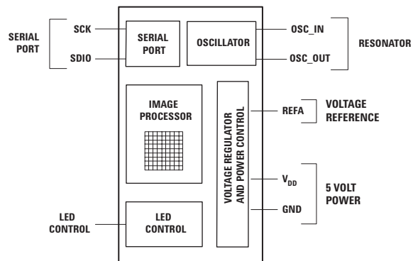
Figure 6. Block diagram of ADNS-2610 optical mouse sensor.
